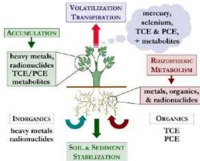
Figure 2: Phytoremediation Mechanism
